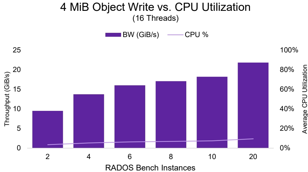
Figure 10 – 4 MiB Object Write Throughput vs. Average CPU Utilization
