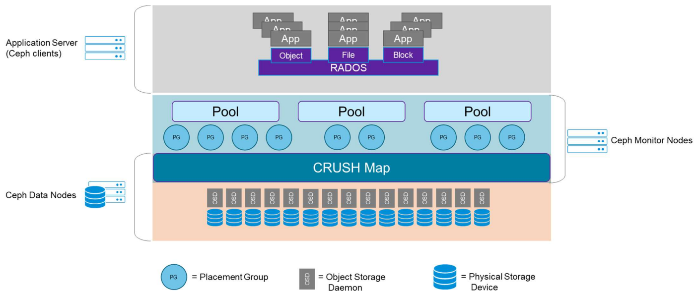
Figure 1 - Ceph Architecture
