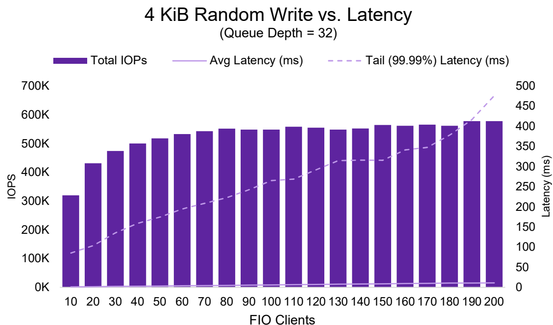
Figure 3 – 4 KiB Random Write IOPS vs. Latency
