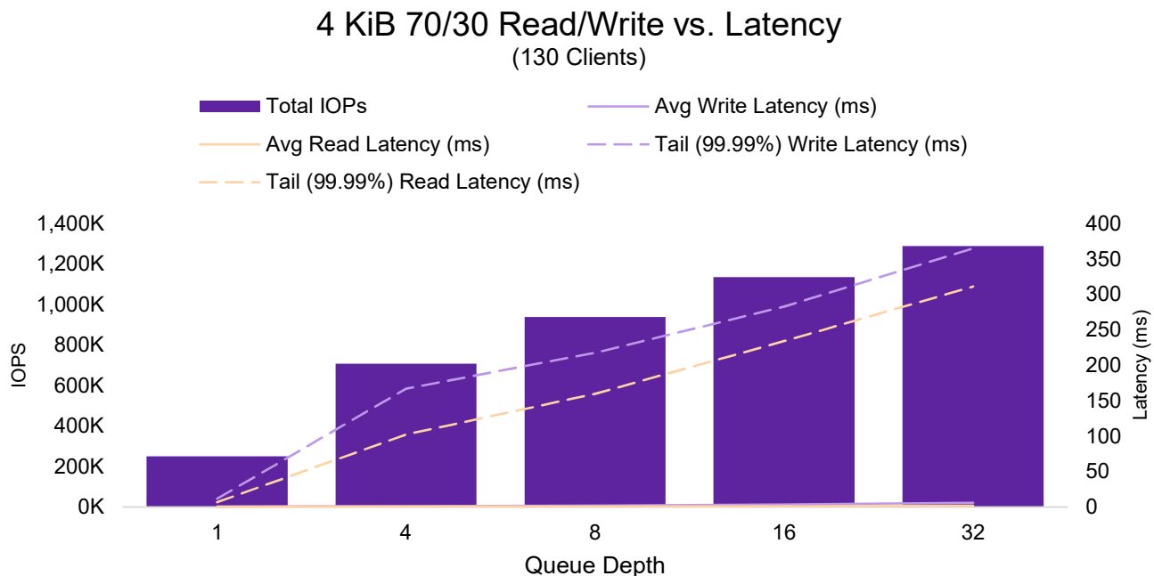
Figure 7 - 4 KiB Random 70/30 Read/Write IOPS vs. Latency
