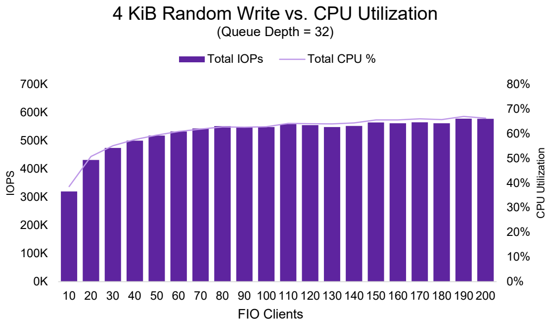
Figure 4 – 4 KiB Random Write IOPS vs. CPU Utilization
