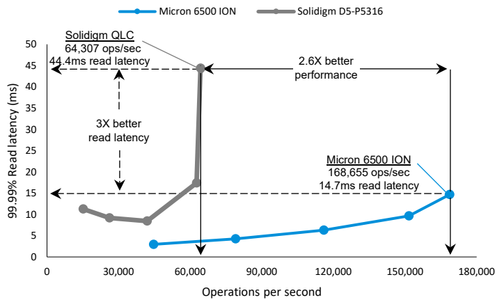
Figure 4: Workload C performance vs. latency
