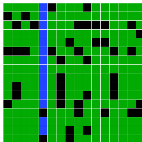
Figure 4: Garbage collection example with typical data center SSD over-provisioning
