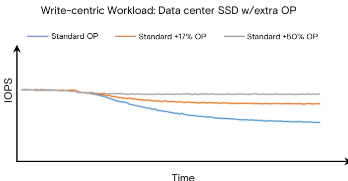
Figure 5: Effects of additional OP in a data center SSD 6
