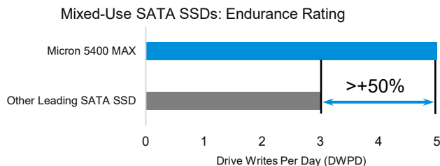
Figure 2b: Mixed-use SSD endurance comparison
