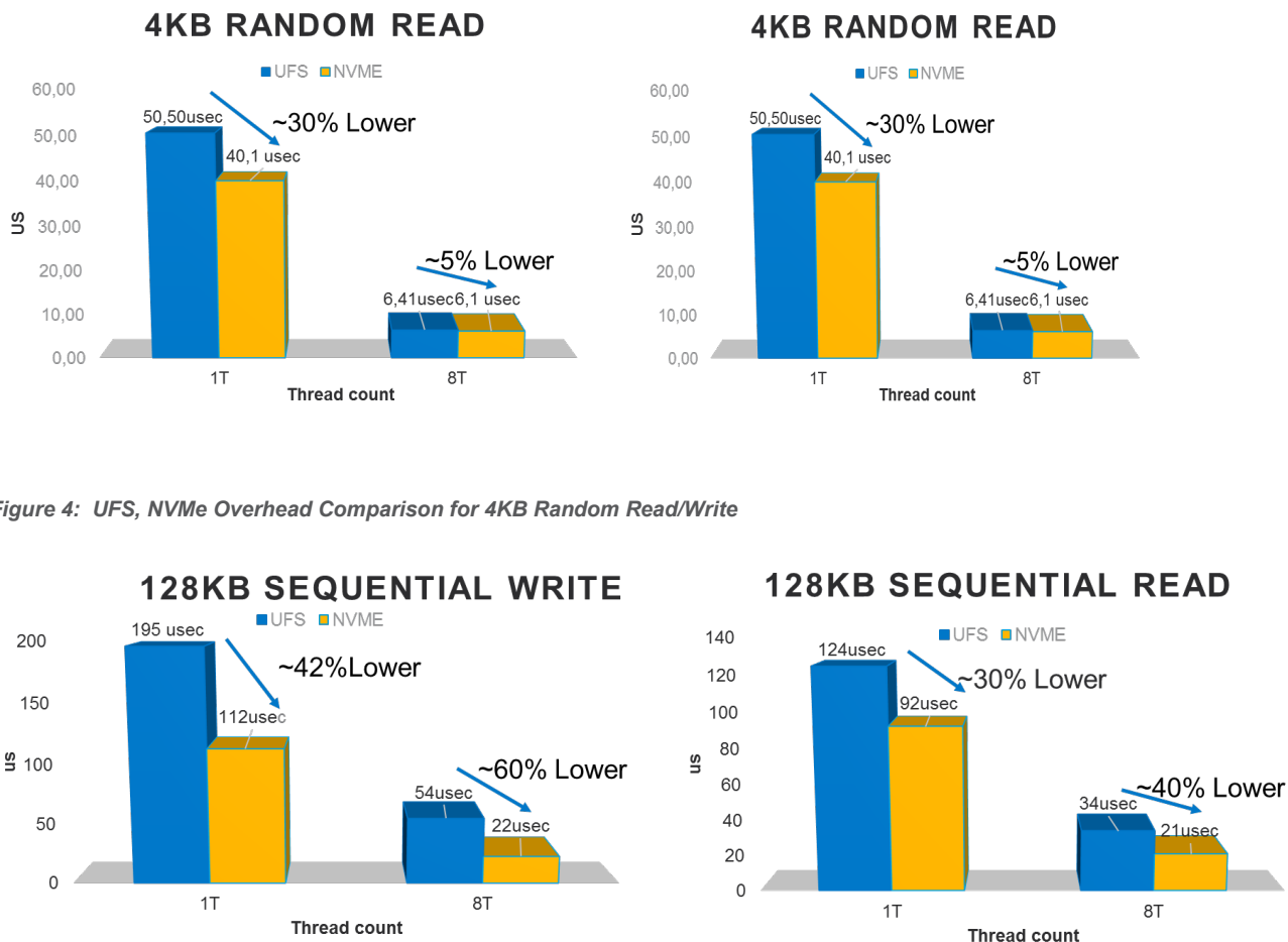
Figure 5: UFS, NVMe Overhead Comparison for 128KB Sequential Read/Write
