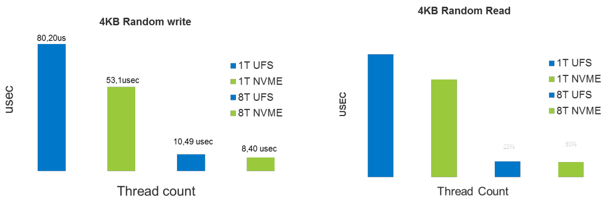
Figure 2. IO Duration Breakdown for 4KB Random Write/Read
