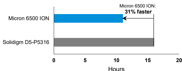
Figure 11b: Cluster rebuild time with load
